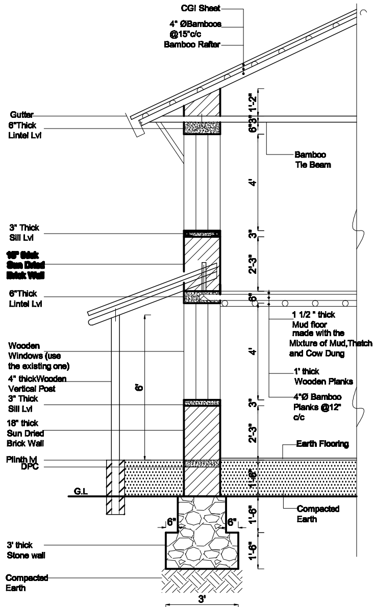
WALL DETAILING
