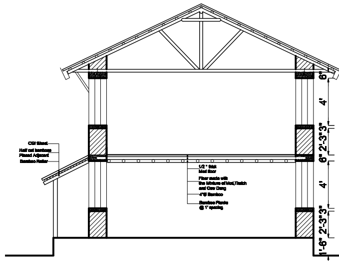
SECTION AT B-B
