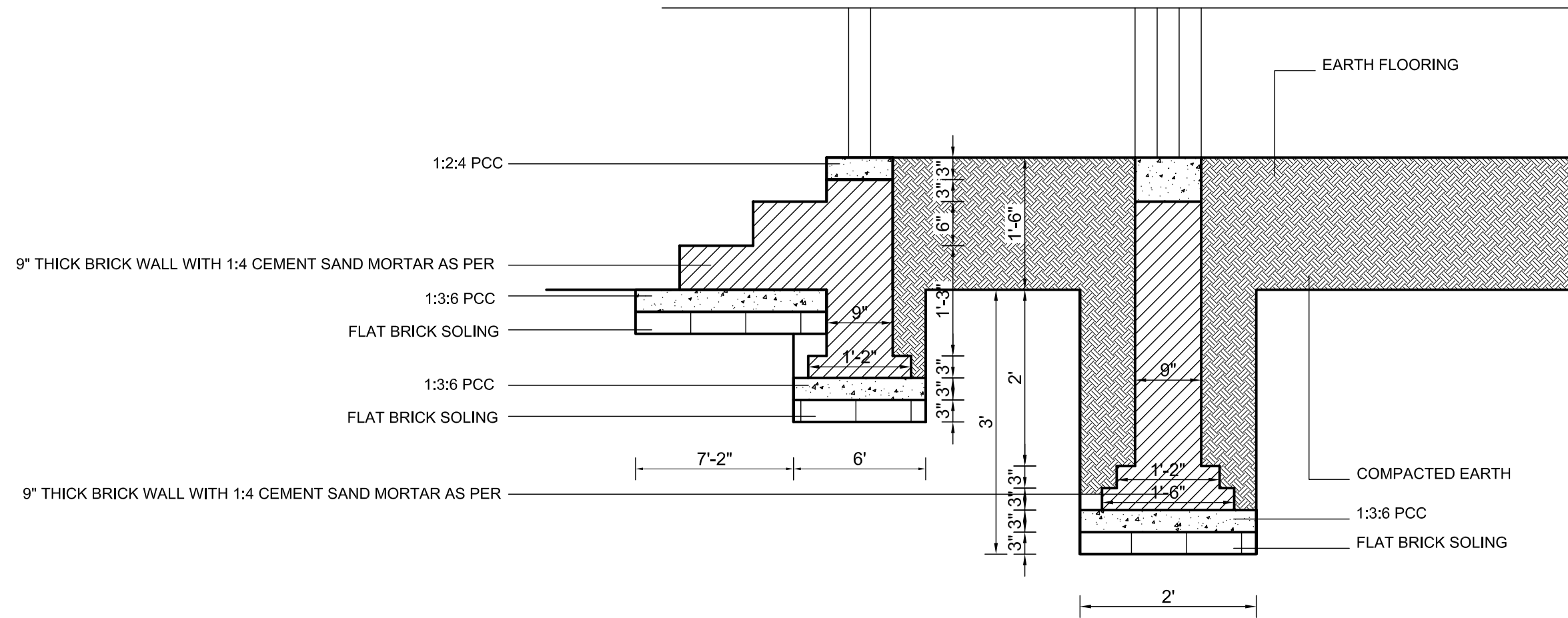
DETAIL AT B
