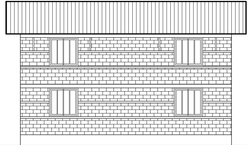
BACK ELEVATION
